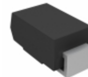
SMAJ58CA-M3/61 Vishay Semiconductor Diodes Division TVS DIODE 58VWM 93.6VC DO-214AC
