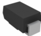
SMAJ58CA-E3/61 Vishay Semiconductor Diodes Division TVS DIODE 58VWM 93.6VC SMA
