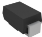
SMAJ58CA-M3/5A Vishay Semiconductor Diodes Division TVS DIODE 58VWM 93.6VC DO-214AC
