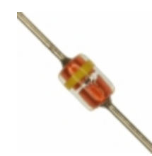
MTZJT-727.5C Rohm Semiconductor DIODE ZENER 7.5V 500MW DO34
