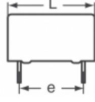
B32676G8685K EPCOS (TDK) CAP FILM 6.8UF 10% 875VDC RADIAL
