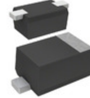
DB2S20500L Panasonic Electronic Components DIODE SCHOTTKY 15V 200MA SSMINI2
