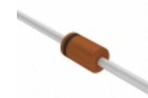
MTZJ9V1SA R0G TSC (Taiwan Semiconductor) DIODE ZENER 8.51V 500MW DO34
