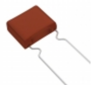
ECW-F2184JAB Panasonic Electronic Components CAP FILM 0.18UF 5% 250VDC RADIAL
