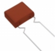
ECW-F2184JAQ Panasonic Electronic Components CAP FILM 0.18UF 5% 250VDC RADIAL
