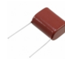
ECQ-E6225JFB Panasonic Electronic Components CAP FILM 2.2UF 5% 630VDC RADIAL
