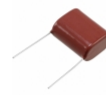
ECQ-E6225KF Panasonic Electronic Components CAP FILM 2.2UF 10% 630VDC RADIAL
