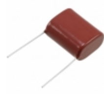
ECQ-E6225KFW Panasonic Electronic Components CAP FILM 2.2UF 10% 630VDC RADIAL
