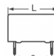
B32796G4136K EPCOS (TDK) CAP FILM 13UF 10% 1.05KVDC RAD
