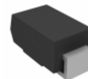
BZG03C130-HM3-18 Electro-Films (EFI) / Vishay DIODE ZENER 130V 1.25W DO214AC
