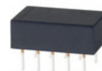
TQ2-5V-3 Panasonic Electric Works RELAY TELECOM DPDT 1A 5V
