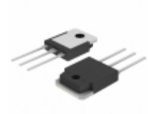
TIP35CP STMicroelectronics TRANS NPN 100V 25A TO-3P
