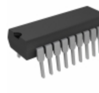
PIC16LC620-04E/P Microchip Technology IC MCU 8BIT 896B OTP 18DIP
