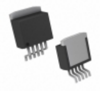
LT1963AEQ-1.8#TRPBF ADI (Analog Devices, Inc.) IC REG LINEAR 1.8V 1.5A 5DDPAK
