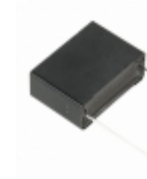
ECQ-UAAF155K Panasonic Electronic Components CAP FILM 1.5UF 10% 275VAC RADIAL
