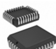
AT29C020-10JI Microchip Technology IC FLASH 2MBIT 100NS 32PLCC
