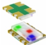
LNJ757W86RA Panasonic Electronic Components LED RGB 628NM 525NM 470NM 4SMD
