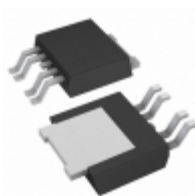
BA03CC0WFP-E2 Rohm Semiconductor IC REG LDO 3V 1A TO252-5
