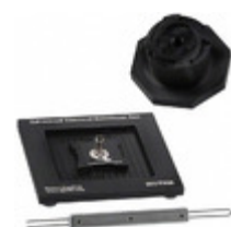
MGT325 Advanced Thermal Solutions, Inc. TOOL FOR MAXI GRIP 32.5X32.5
