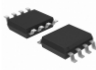
11LC020-E/SN Microchip Technology IC EEPROM 2KBIT 100KHZ 8SOIC
