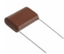
ECQ-E6824JFW Panasonic Electronic Components CAP FILM 0.82UF 5% 630VDC RADIAL
