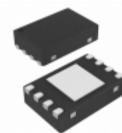
CM1431-04DE ON Semiconductor FILTER RC(PI) 100 OHM/15PF SMD
