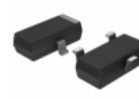
BC858AMTF Fairchild/ON Semiconductor TRANS PNP 30V 0.1A SOT-23
