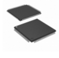
LCMXO2280E-4T144I Lattice Semiconductor Corporation IC FPGA 113 I/O 144TQFP
