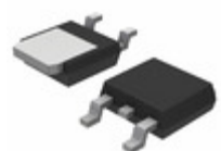
MC78M15ABDT ON Semiconductor IC REG LDO 15V 0.5A DPAK
