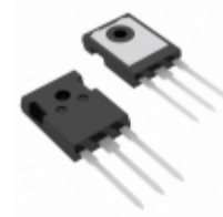
IXGH30N60B IXYS IGBT 600V 60A 200W TO247AD
