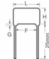
ECQ-P1H391JZ3 Panasonic Electronic Components CAP FILM 390PF 5% 50VDC RADIAL
