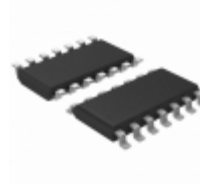
74VHC86M Fairchild/ON Semiconductor IC GATE XOR 4CH 2-INP 14-SOIC
