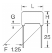
ECQ-P6222JU Panasonic Electronic Components CAP FILM 2200PF 5% 630VDC RADIAL
