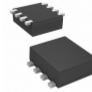
FC8V22040L Panasonic Electronic Components MOSFET 2N-CH 24V 8A WMINI8-F1
