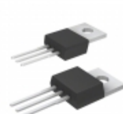
BUL44 ON Semiconductor TRANS NPN 400V 2A TO-220AB
