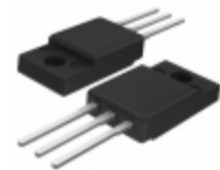
BT138X-800F,127 WeEn Semiconductors TRIAC 800V 12A TO220-3
