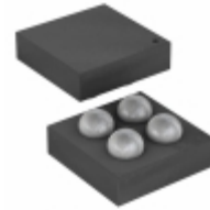
AT24CSW080-UUM0B-T Microchip Technology IC EEPROM 8KBIT 1MHZ 4WLCSP
