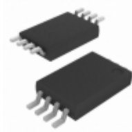
AT24HC02B-TH-B Microchip Technology IC EEPROM 2KBIT 1MHZ 8TSSOP
