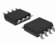
PIC12F609T-I/SN Microchip Technology IC MCU 8BIT 1.75KB FLASH 8SOIC
