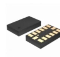
LSM303DLHCTR STMicroelectronics IMU ACCEL/MAG 3-AXIS I2C 14LGA
