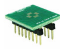
PA0060 Chip Quik, Inc. QFN-16-THIN TO DIP-16 SMT ADAPTE
