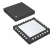
PIC16F913-E/ML Microchip Technology IC MCU 8BIT 7KB FLASH 28QFN
