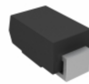
SMAJ14C-E3/61 Vishay Semiconductor Diodes Division TVS DIODE 14VWM 25.8VC SMA
