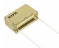
PME271MD6220KR30 KEMET CAP FILM 0.22UF 10% 630VDC RAD
