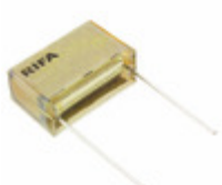
PME271MD6100MR30 KEMET CAP FILM 0.1UF 20% 630VDC RADIAL
