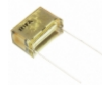
PME271M622KR30 KEMET CAP FILM 0.22UF 20% 275VAC RAD
