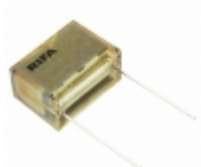
PME271M647KR30 KEMET CAP FILM 0.47UF 10% 275VAC RAD
