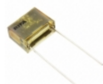
PME271MB6100KR30 KEMET CAP FILM 0.1UF 10% 275VAC RADIAL
