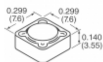
DR73-821-R Bussmann (Eaton) FIXED IND 820UH 270MA 3.93 OHM
