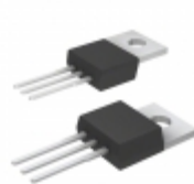
IXSP10N60B2D1 IXYS IGBT 600V 20A 100W TO220AB
