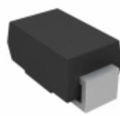
P4SMA12AHE3/61 Electro-Films (EFI) / Vishay TVS DIODE 10.2V 16.7V DO214AC
