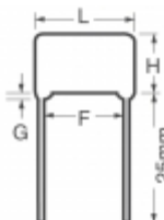
ECQ-P1H271JZ3 Panasonic Electronic Components CAP FILM 270PF 5% 50VDC RADIAL
