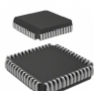
CY7C131-15JXI Cypress Semiconductor IC SRAM 8KBIT 15NS 52PLCC
