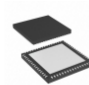
PIC32MZ0512EFE064-I/MR Microchip Technology IC MCU 32BIT 512KB FLASH 64QFN
