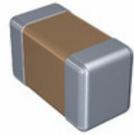
C0603C101J4GAC7867 KEMET CAP CER 100PF 16V NP0 0603
