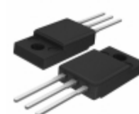
BTA202X-800E,127 WeEn Semiconductors TRIAC SENS GATE 800V 2A TO220-3
