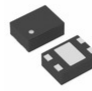
XC6108N26BGR-G Torex Semiconductor Ltd IC SUPERVISOR 2.6V 4-USP
