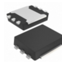
S-1135D27-A6T1U SII Semiconductor Corporation IC REG LINEAR 2.7V 0.3A HSNT-6A
