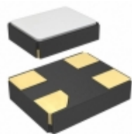
CX3225SB30000D0FPLCC AVX Corporation CRYSTAL 30.0000MHZ 8PF SMD
