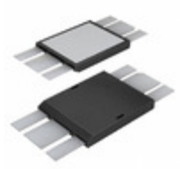
IXFZ520N075T2 IXYS MOSFET N-CH 75V 465A DE-475
